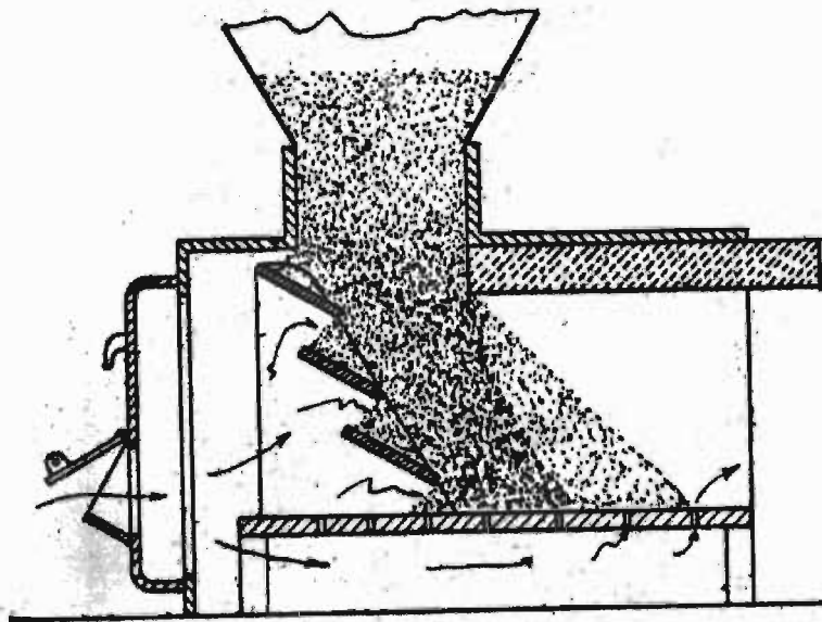
SECTION SHOWING TYPICAL MULTIPLE SHELF FEED GRATES.
