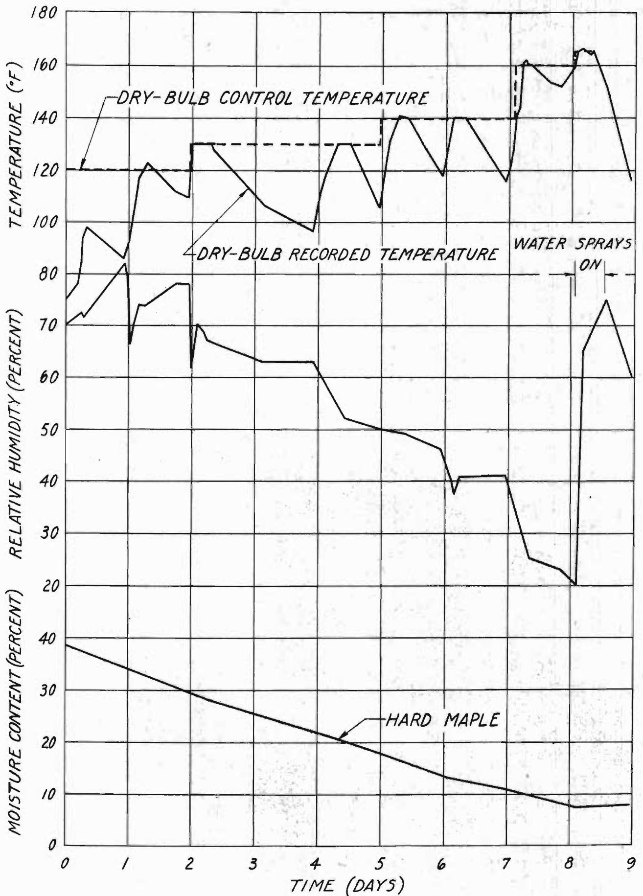
Figure 4.--Drying conditions in furnace-type lumber dry kiln and resulting drying rate of commercial hard maple.
