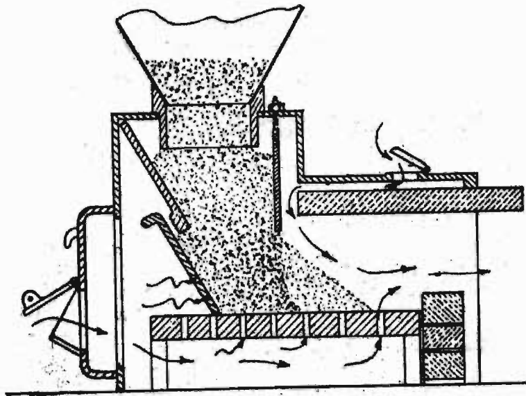
SECTION SHOWING TYPICAL TWO-PIECE FEED GRATE.
