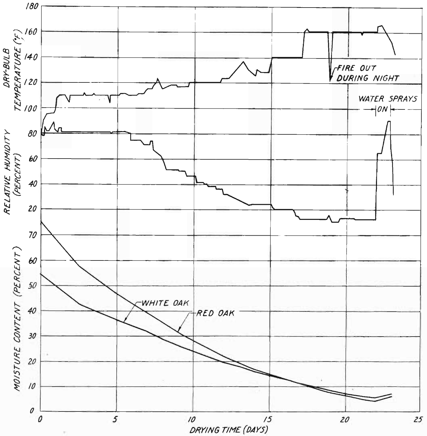
Figure 3.--Drying conditions in furnace-type lumber dry kiln and resulting drying rate of commercial white and red oak.
